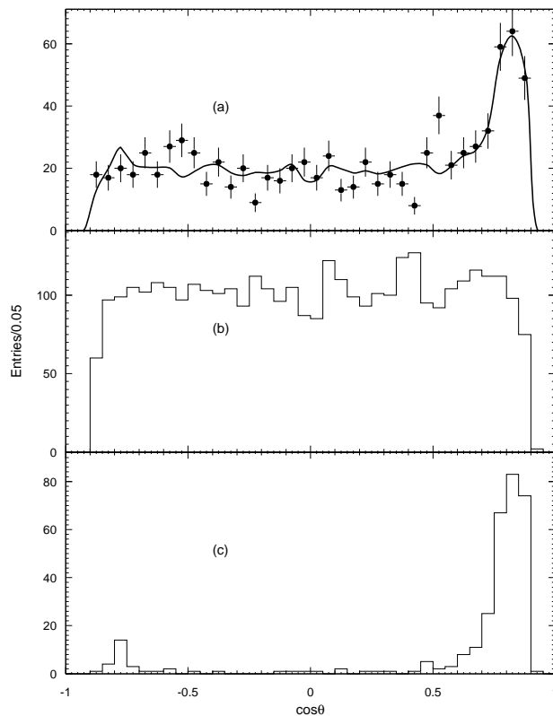
Figure 1: Determination of the remaining Bhabha contribution in the final e-e sample for 1994-1995 data: \cos\theta^* distributions for (a) data, (b) \tau\tau simulation, and (c) Bhabha simulation. The solid line represents a fit of the data with the relative normalization of the \tau\tau and Bhabha contributions left free.
