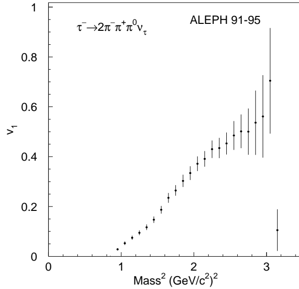
Figure 55: The spectral function for the 3\pi\pi^0 hadronic mode. While the original spectral function is determined in 0.025 \text{ GeV}^2 bins, it is rebinned here to 0.1 \text{ GeV}^2 for easier reading.
