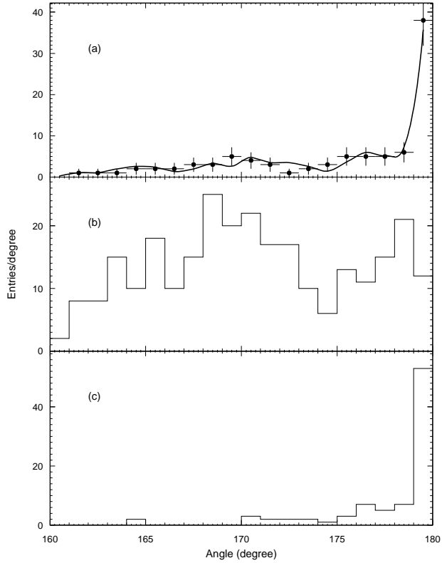
Figure 3: Determination of the remaining \gamma^*\gamma^* \rightarrow \mu^+\mu^- contribution in the final \mu\text{-}\mu sample for 1994-1995 data: acoplanarity angle distributions for (a) data, (b) \tau\tau simulation, and (c) e^+e^- \rightarrow (e^+e^-)\mu^+\mu^- simulation. The solid line represents a fit of the data with the relative normalization of the \tau\tau and \gamma\gamma -induced \mu -pair contributions left free.
