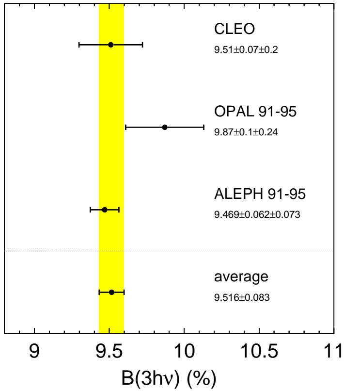
Figure 46: Comparison of ALEPH measurement with published precise results from other experiments for \tau \rightarrow 3h\nu (sum of 3\pi\nu , K2\pi\nu and 2K\pi\nu ). References for other experiments are CLEO [39], OPAL [40].
