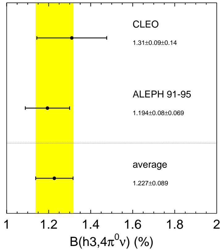
Figure 45: Comparison of ALEPH measurement with published precise results from other experiments for \tau \rightarrow h(3, 4)\pi^0\nu (sum of \pi(3, 4)\pi^0\nu and K(3, 4)\pi^0\nu ). References for other experiments are CLEO [38].
