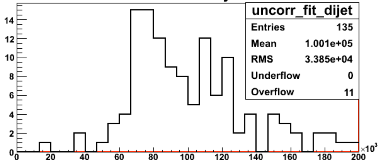
Uncorrected and fitted dijet distribution
