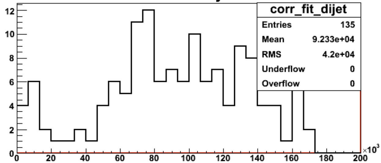
Corrected and fitted dijet distribution
